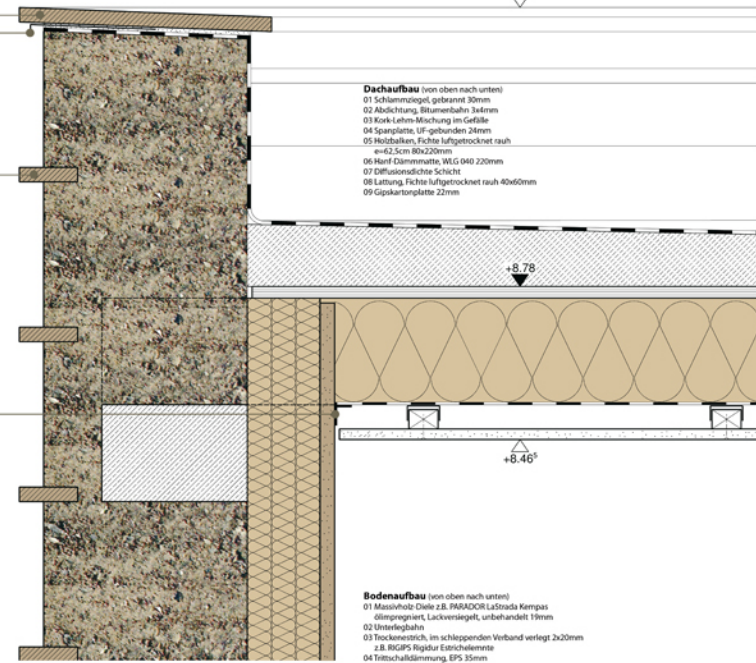
Detail 4 M 1:5
